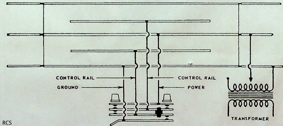
Wiring Diagram of Remote Control Set Type RCS
